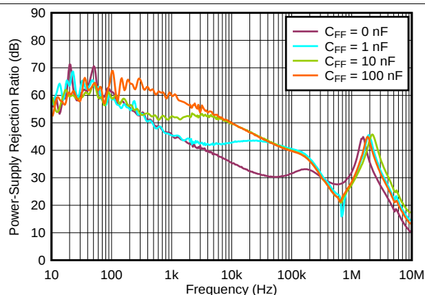
Figure 32. PSRR vs Frequency and C_{FF}
