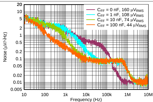
Figure 34. Output Spectral Noise Density
