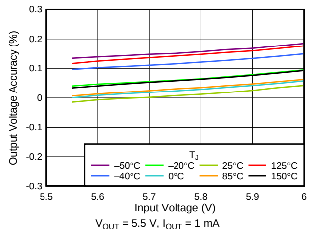
Figure 3. 5.5-V Line Regulation vs V_{IN}
