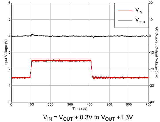
Figure 5-14. Line Transient
