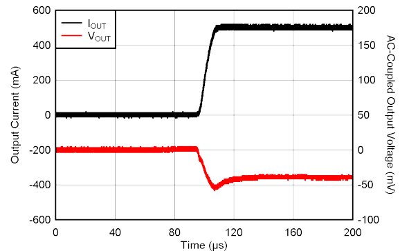
Figure 5-10. Current Limit
