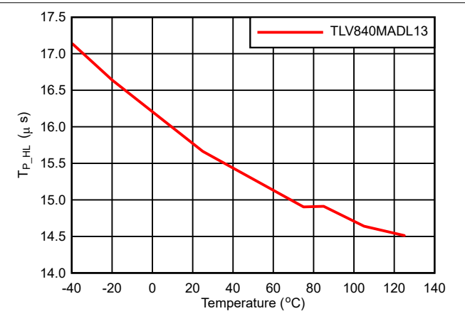
Figure 7-7. Propagation Delay vs Temperature
