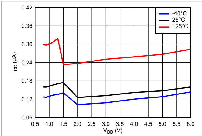
Figure 7-4. Supply Current vs Supply Voltage
