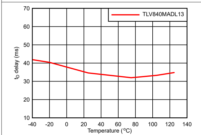
Figure 7-8. Reset Time Delay vs Temperature
