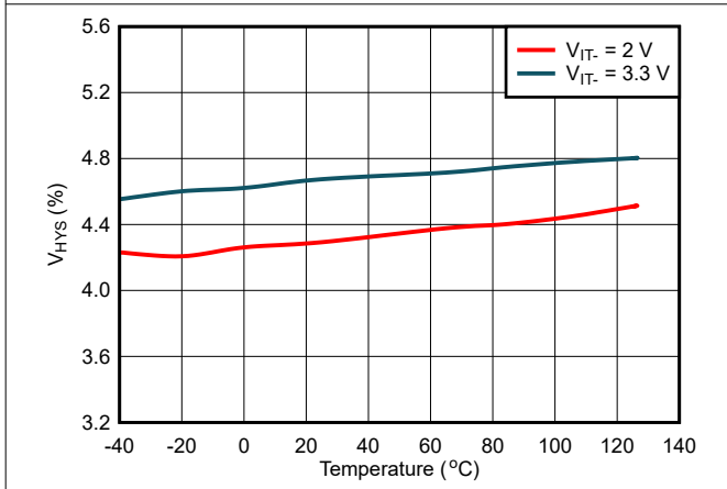
Figure 7-6. V_{HYS} vs Temperature
