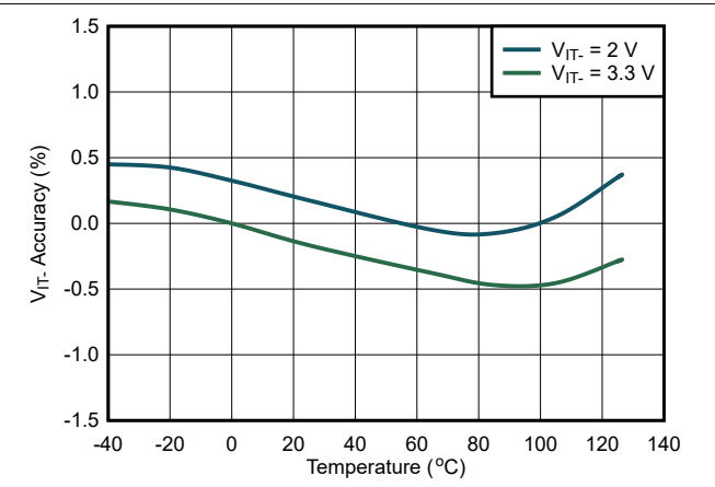
Figure 7-5. V_{IT-} Accuracy vs Temperature
