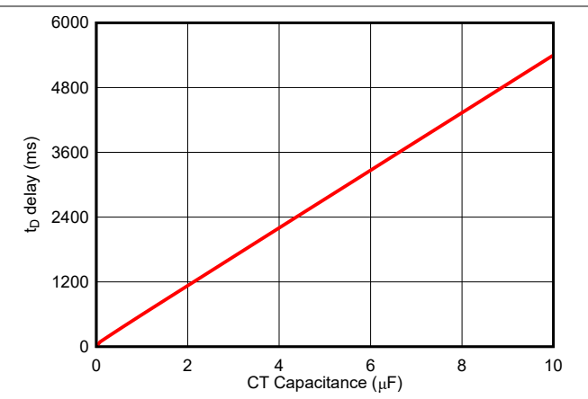
Figure 7-9. Reset Time Delay vs C_T Capacitance
