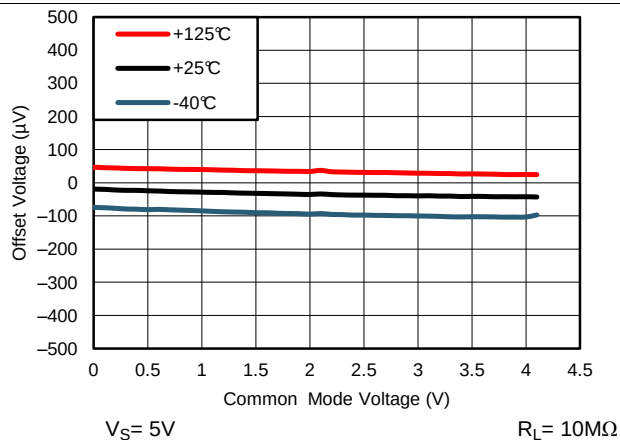
Figure 5. Typical Offset Voltage vs. Common Mode Voltage
