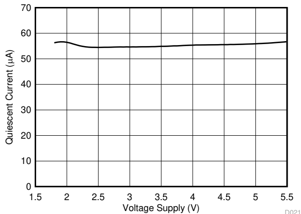
Figure 6-21. Quiescent Current vs Supply Voltage
