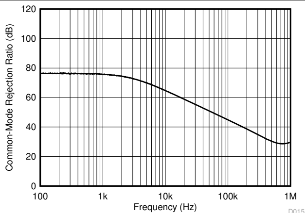
Figure 6-15. CMRR vs Frequency
