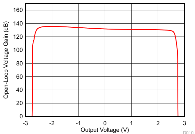
Figure 6-10. Open-Loop Gain vs Output Voltage
