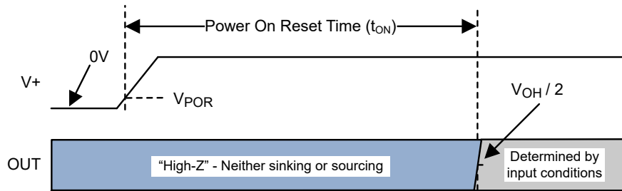
Figure 6-2. TLV903xL1-Q1 Power-On Reset Timing Diagram Example
