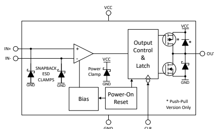
Simplified Block Diagram
