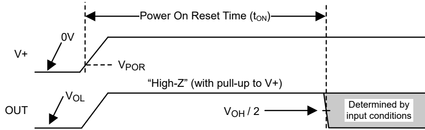
Figure 6-1. TLV902xL1-Q1 Power-On Reset Timing Diagram Example
