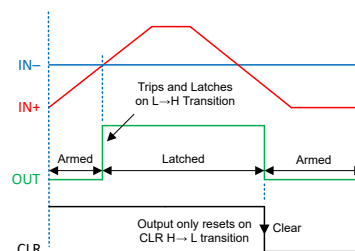
TLV903xL-Q1 Push-Pull Latching Response
