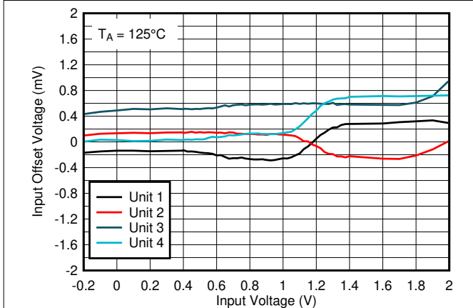
Figure 5-23. Offset Voltage vs Input Voltage at 125^\circ\text{C} , 1.8V
