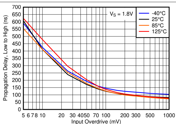
Figure 5-18. Propagation Delay, Low to High, 1.8V
