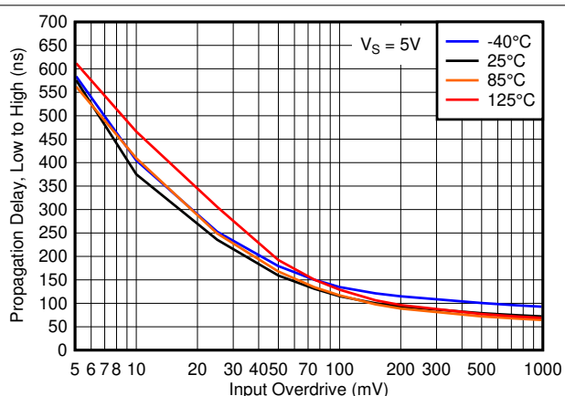
Figure 5-22. Propagation Delay, Low to High, 5V
