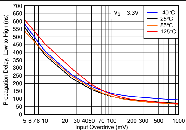
Figure 5-20. Propagation Delay, Low to High, 3.3V
