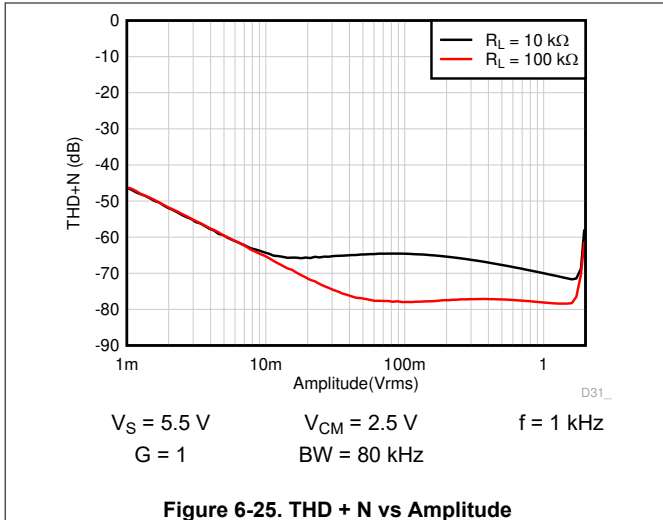
Figure 6-25. THD + N vs Amplitude
