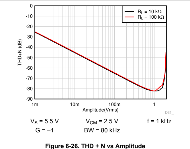
Figure 6-26. THD + N vs Amplitude
