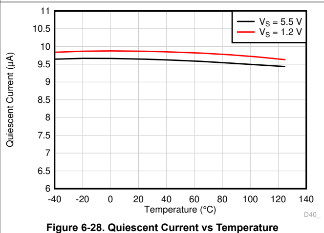
Figure 6-28. Quiescent Current vs Temperature
