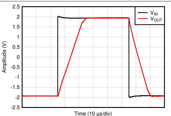
Figure 7-33. Overload Recovery
