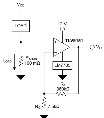
Figure 7-1. TLV9151-Q1 in a Low-Side, Current-Sensing Application
