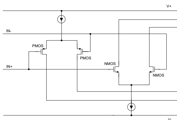
Figure 6-6. Rail-to-Rail Input Stage
