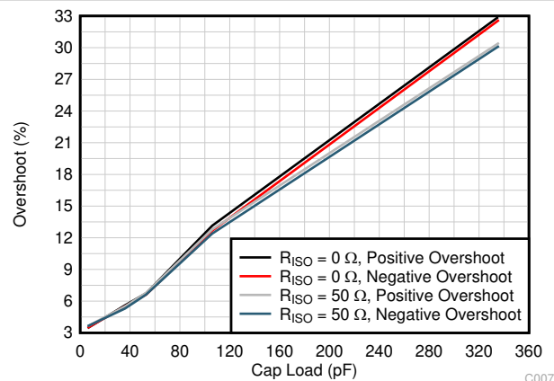
Figure 6-4. Small-Signal Overshoot vs Capacitive Load (10mV Output Step, G = -1)
