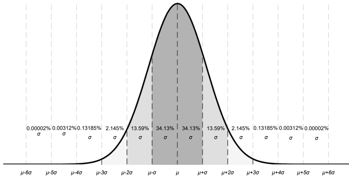
Figure 6-9. Ideal Gaussian Distribution
