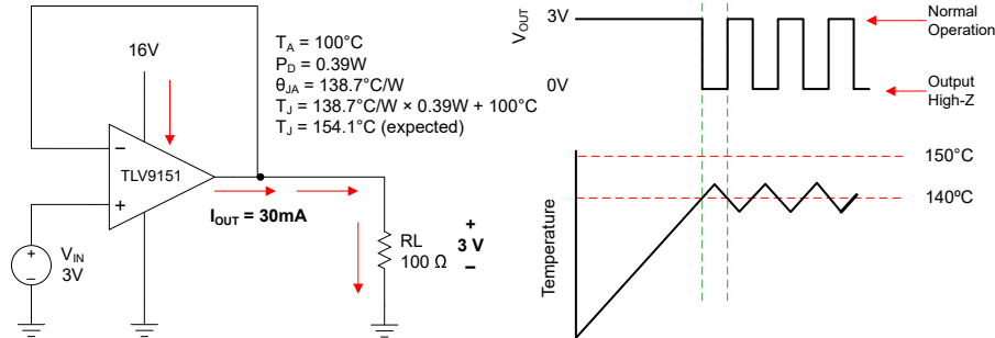
Figure 6-2. Thermal Protection
