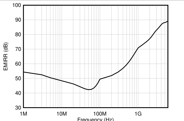
Figure 5-40. EMIRR (Electromagnetic Interference Rejection Ratio) vs Frequency
