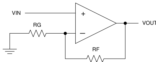
Figure 7-3. Schematic Representation
