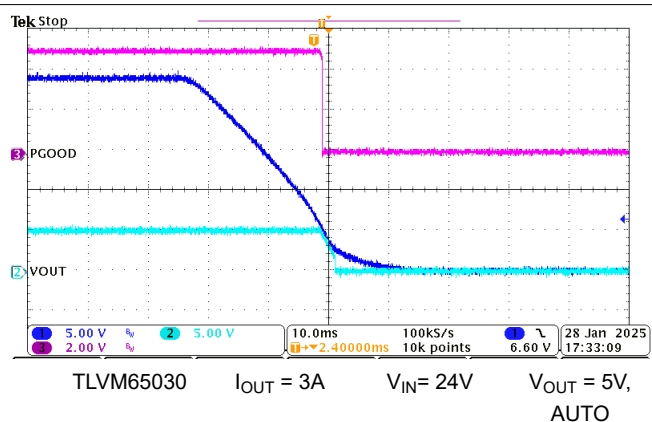
Figure 7-9. Shutdown
