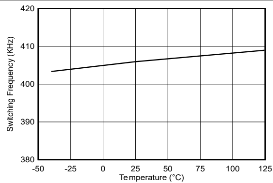
Figure 5-6. f_{SW} 400kHz
