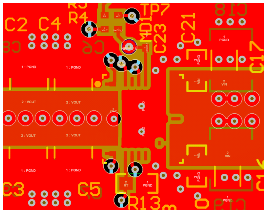
Figure 7-19. Layout Example
