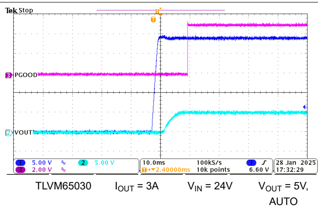
Figure 7-8. Start-Up
