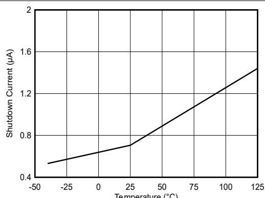
Figure 5-2. Shutdown Input Current
