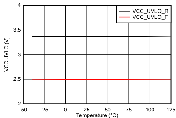
Figure 5-4. VCC UVLO
