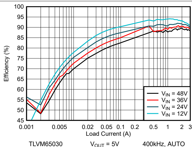
Figure 7-4. Efficiency
