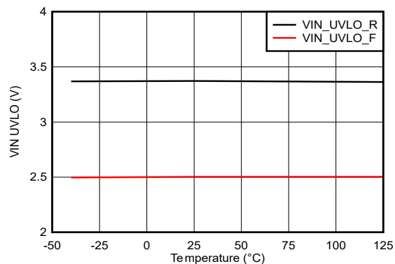
Figure 5-3. Enable UVLO
