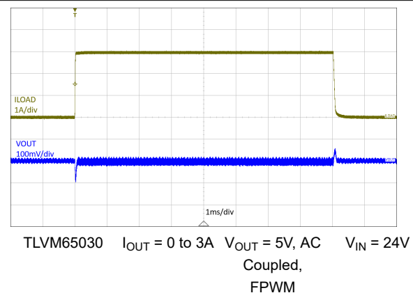
Figure 7-13. Load Transient (0 to 100%)
