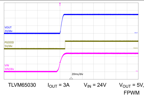
Figure 7-15. Start-Up
