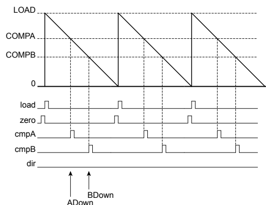
Figure 18-3. PWM Count-Down Mode
