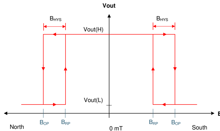
Figure 8-3. Omnipolar Functionality
