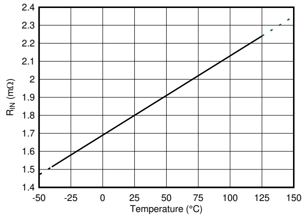
Figure 6-21. Input Conductor Resistance vs Temperature
