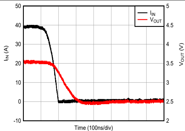
Figure 6-12. Voltage Output Step Response, Falling
