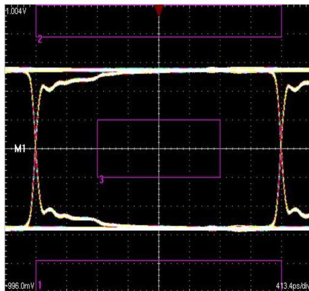
Figure 28. TMDS Data Rate of 302.4 Mbps
