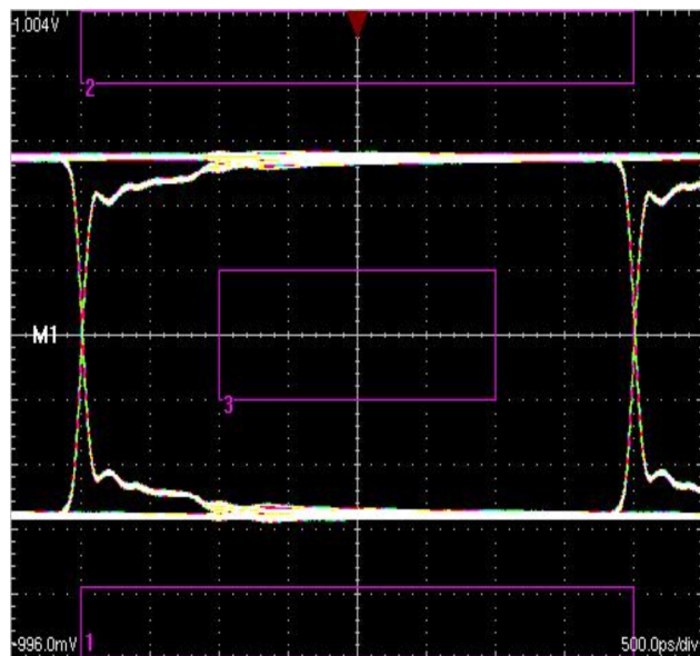
Figure 27. TMDS Data Rate of 250 Mbps
