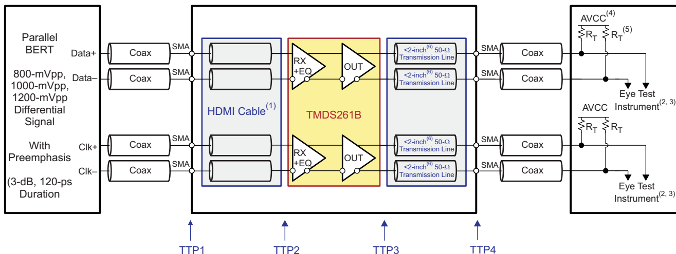
Figure 24. Input Pre-Emphasis Tolerance-Measurement Setup
