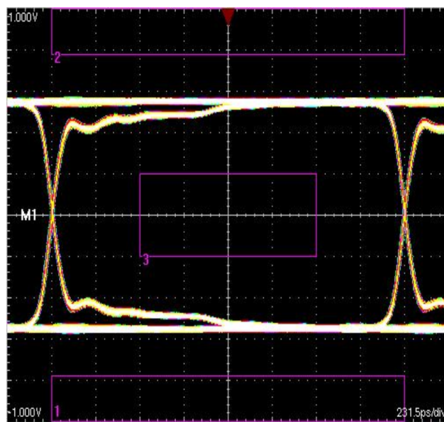
Figure 30. TMDS Data Rate of 540 Mbps
