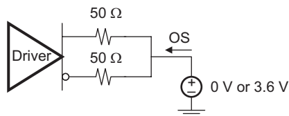
Figure 16. TMDS Main Link Short-Circuit Output Circuit
