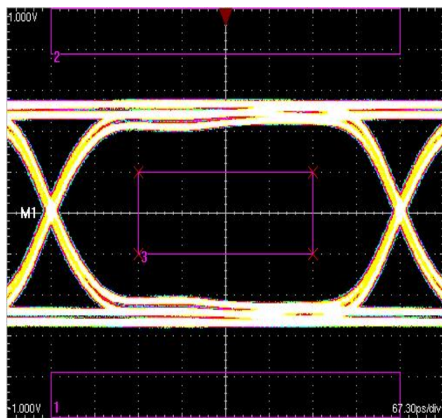
Figure 37. TMDS Data Rate of 1856.25 Mbps
