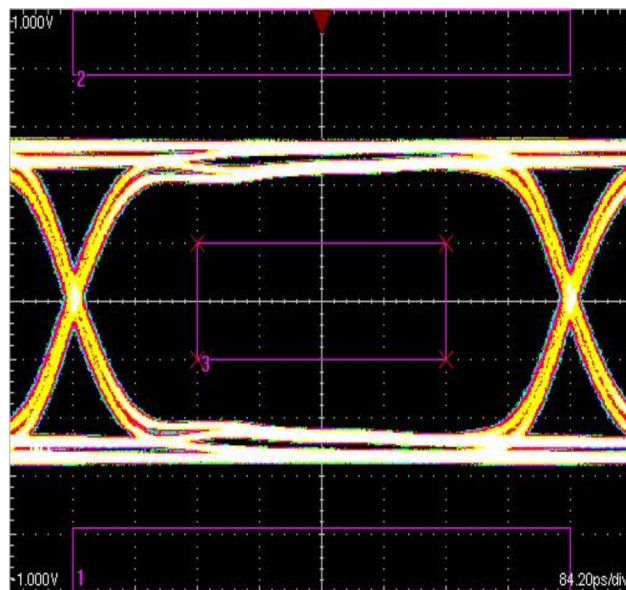
Figure 36. TMDS Data Rate of 1485 Mbps
