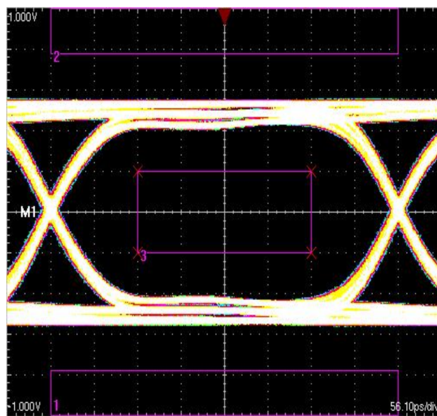
Figure 38. TMDS Data Rate of 2227.5 Mbps
