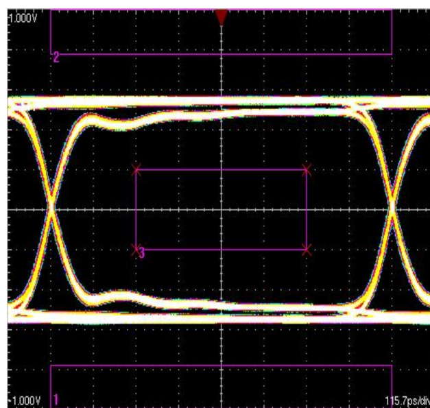
Figure 34. TMDS Data Rate of 1080 Mbps
