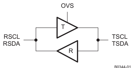
Figure 40. I²C Drivers in the TMD5261B (R Side Is the HDMI Source Side, T Side Is the HDMI Sink Side)
