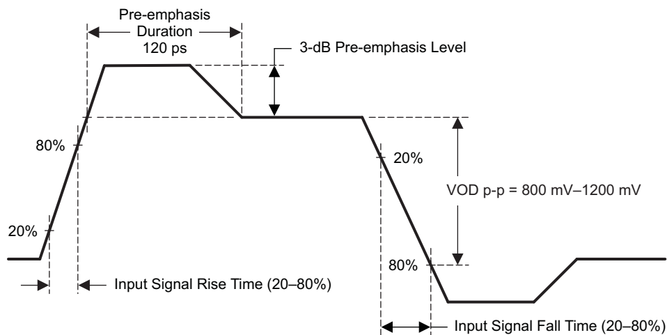
Figure 26. Acceptable Pre-Emphasis Into TMDS361B
