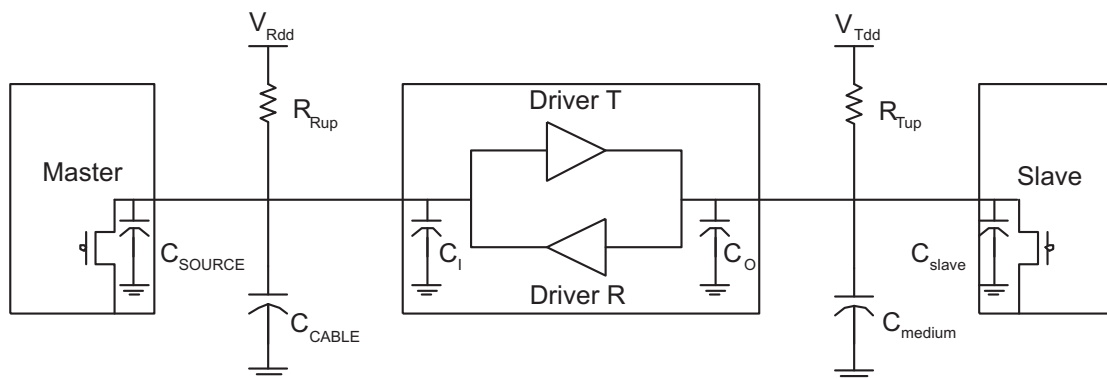
Figure 42. Typical Application
