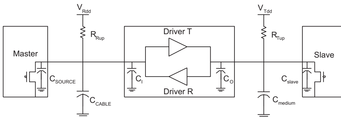
Figure 36. Typical Application
