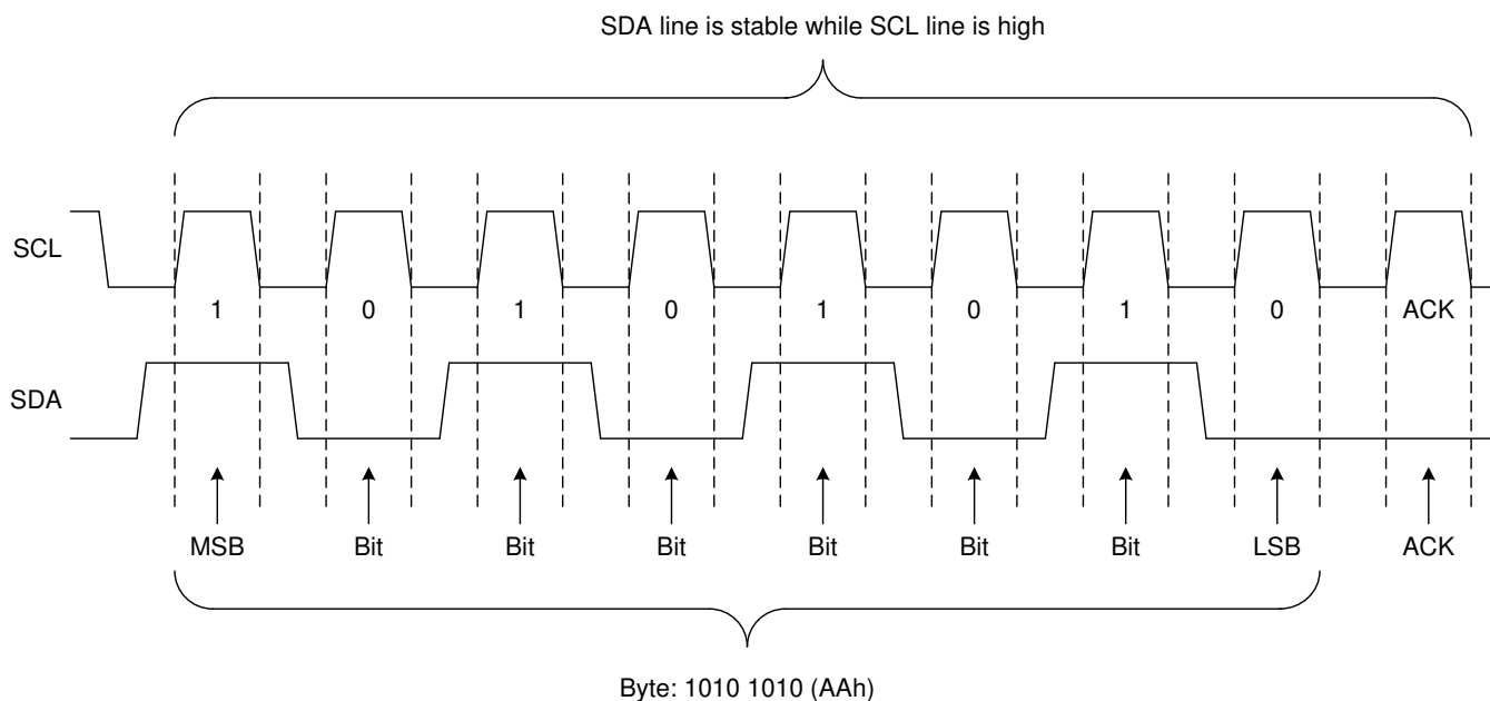
Figure 7-6. Bit Transfer
