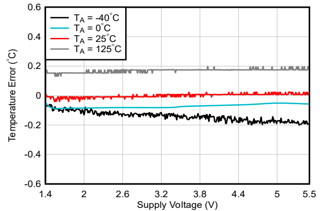
Figure 6-3. Temperature Error vs Supply Voltage
