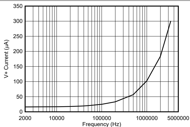
Figure 6-7. Shutdown Quiescent Current vs SCL Clock Frequency
