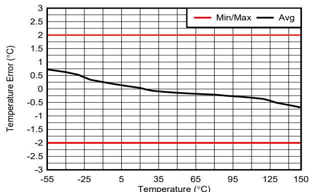
Figure 6-3. Remote Temperature Error vs Device Junction Temperature
