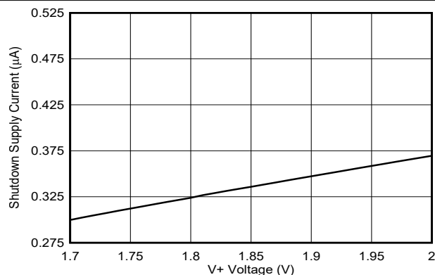
Figure 6-9. Shutdown Quiescent Current vs Supply Voltage
