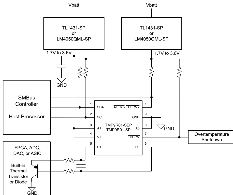
Figure 9-1. TMP9R01-SEP and TMP9R01-SP Basic Connections Using a Processor Built-In Remote Transistor
