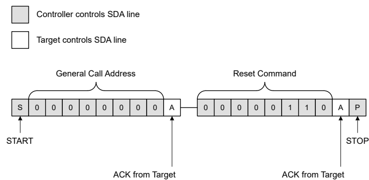
Figure 7-10. SMBus General Call Reset Timing Diagram
