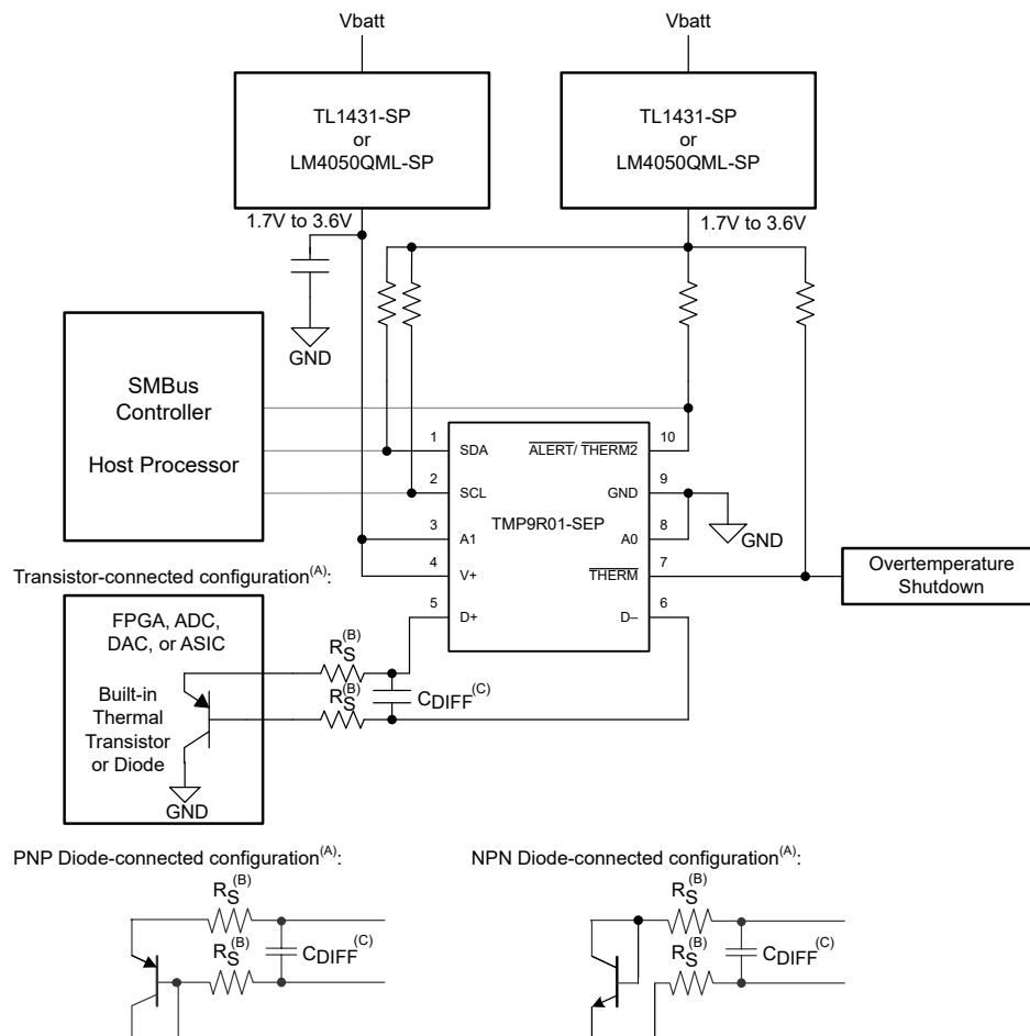
Figure 7-1. Basic Connections
