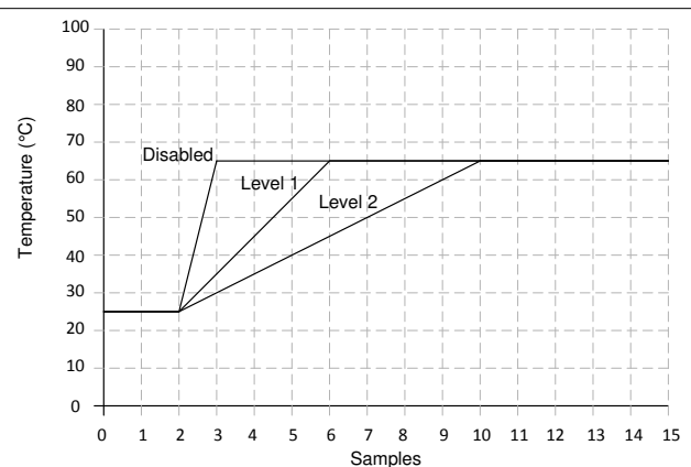
Figure 7-5. Filter Response to Step Inputs
