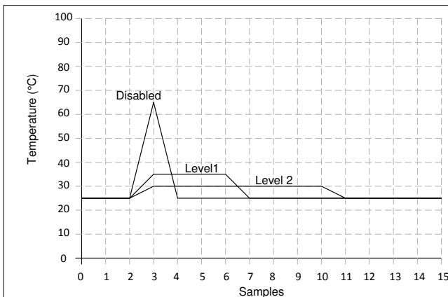
Figure 7-4. Filter Response to Impulse Inputs
