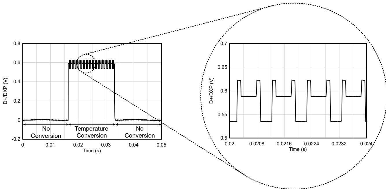
Figure 9-2. D+ Waveform
