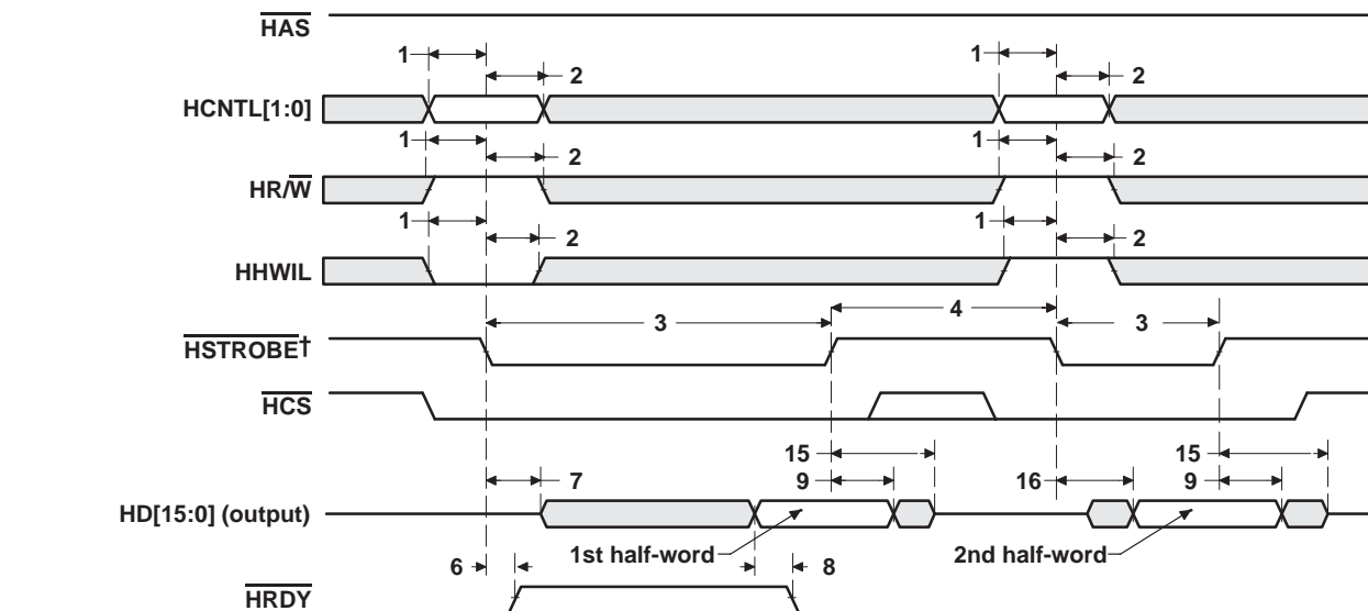
Figure 7-32. HPI16 Read Timing ( \overline{\text{HAS}} Not Used, Tied High)
