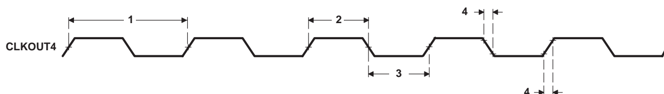
Figure 7–2. CLKOUT4 Timing
