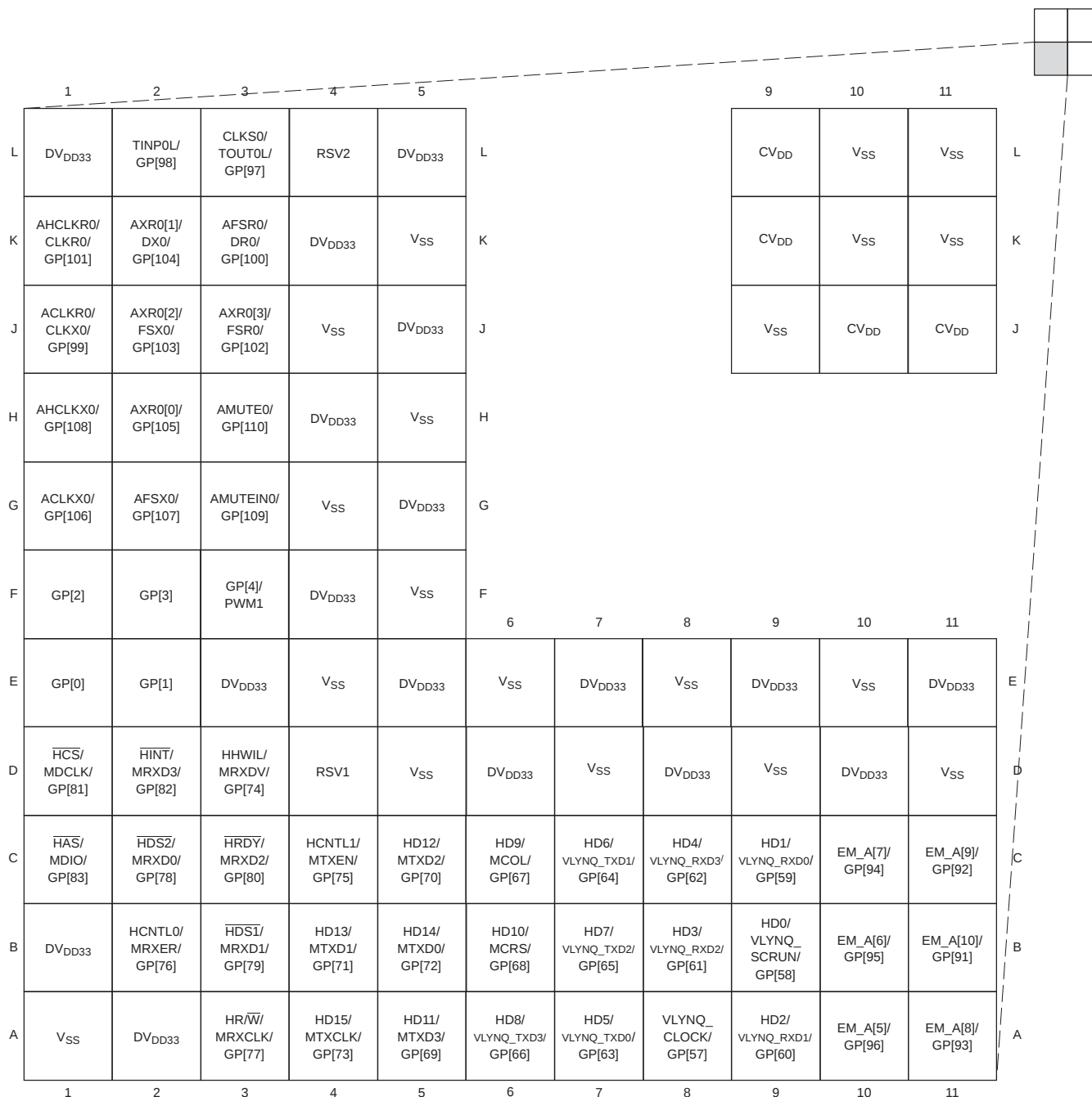
Figure 2-11. ZDU Pin Map [Quadrant D]
