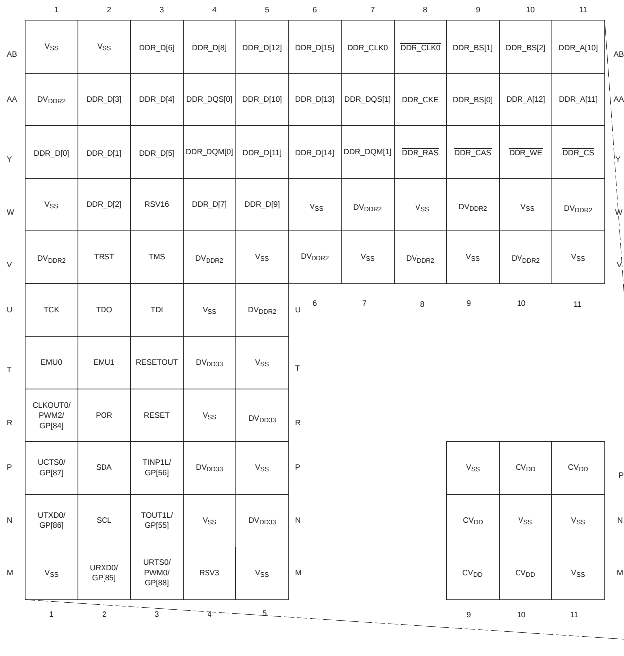
Figure 2-8. ZDU Pin Map [Quadrant A]
