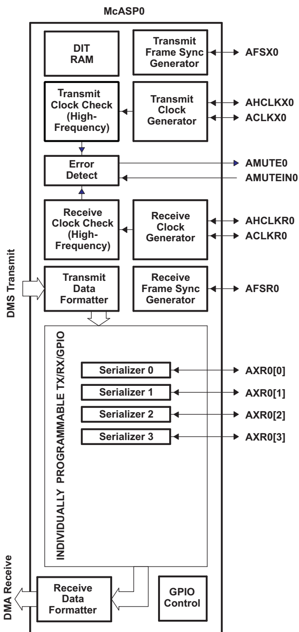
Figure 6-31. McASP0 Configuration
