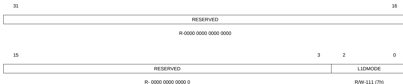
Figure 2-3. L1DCFG Register
