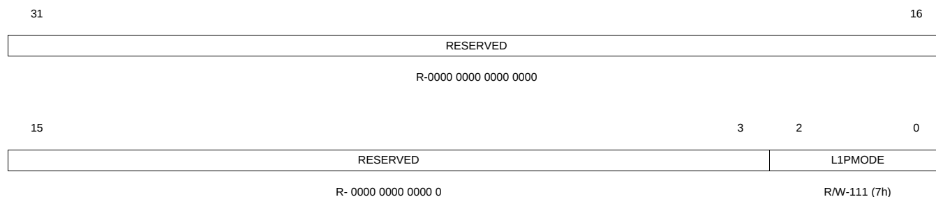
Figure 2-2. L1PCFG Register
