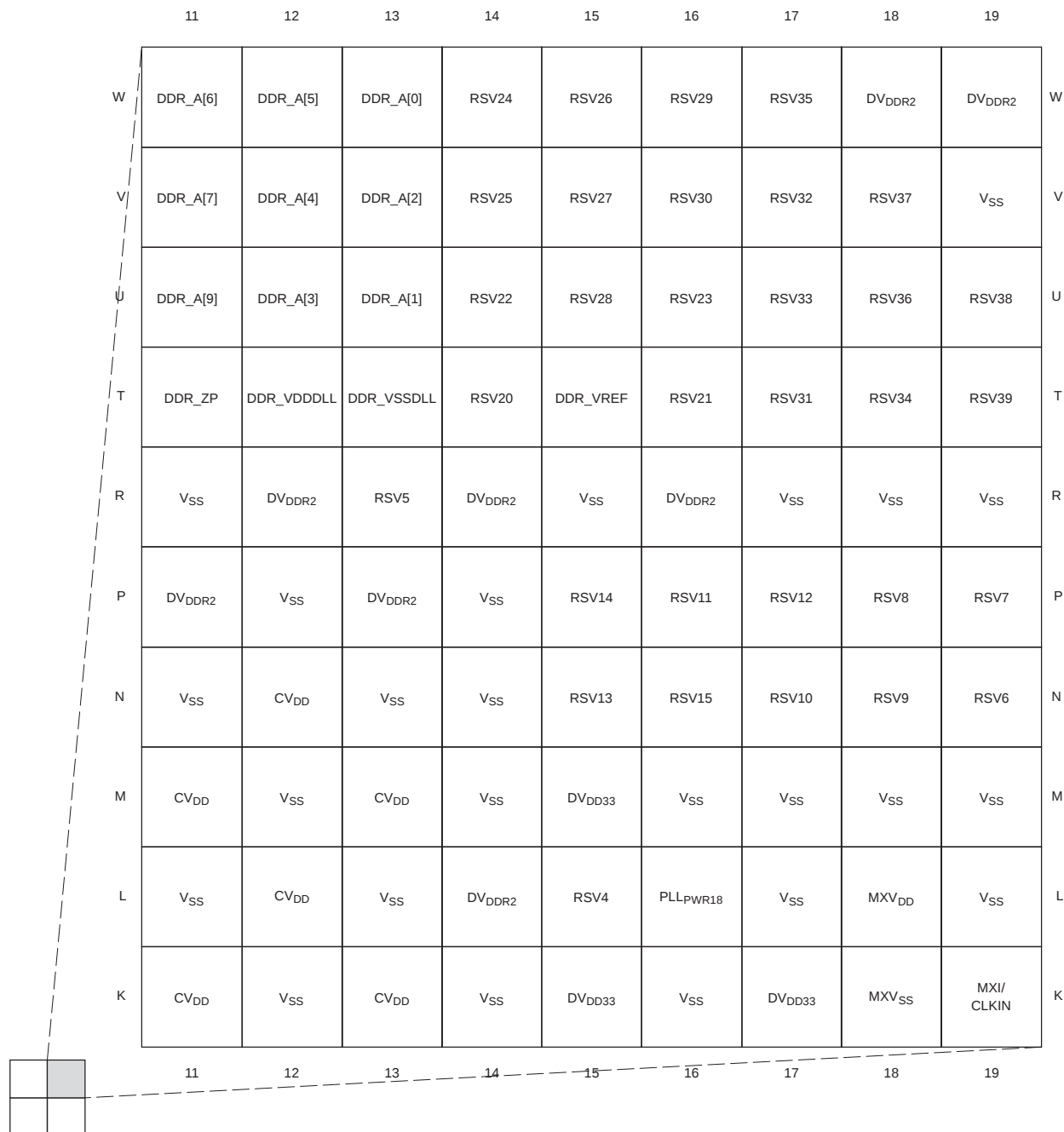
Figure 2-5. ZWT Pin Map [Quadrant B]
