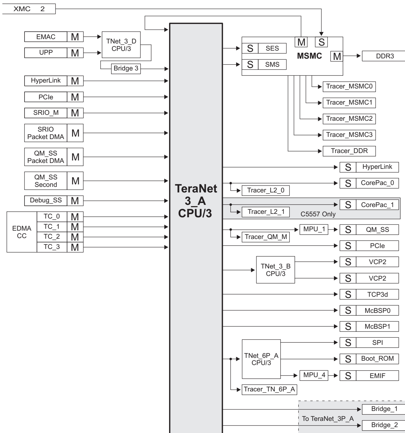
Figure 9-1. TeraNet 3A
