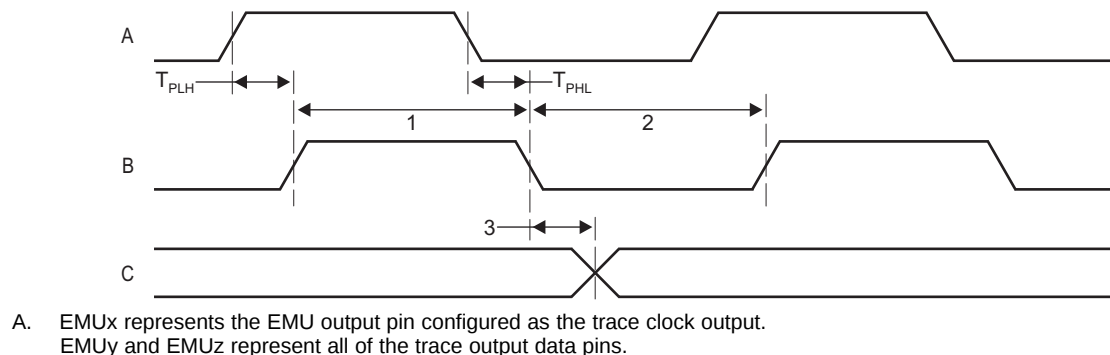
Figure 5-34. Trace Timing
