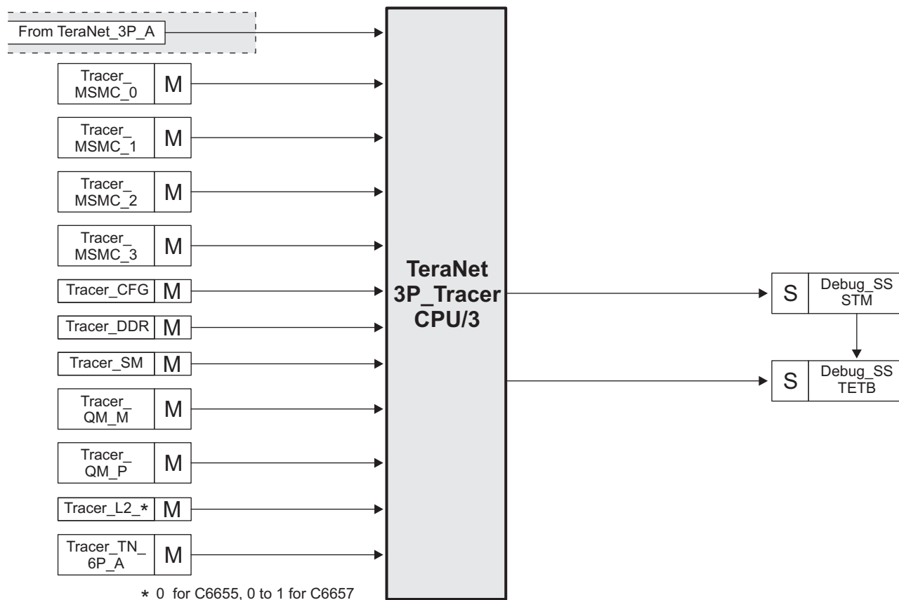
Figure 9-4. TeraNet 3P_Tracer
