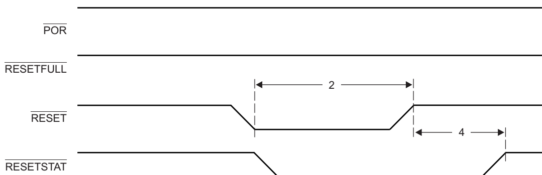
Figure 5-3. Soft/Hard-Reset Timing
