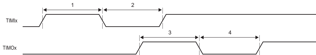
Figure 5-26. Timer Timing
