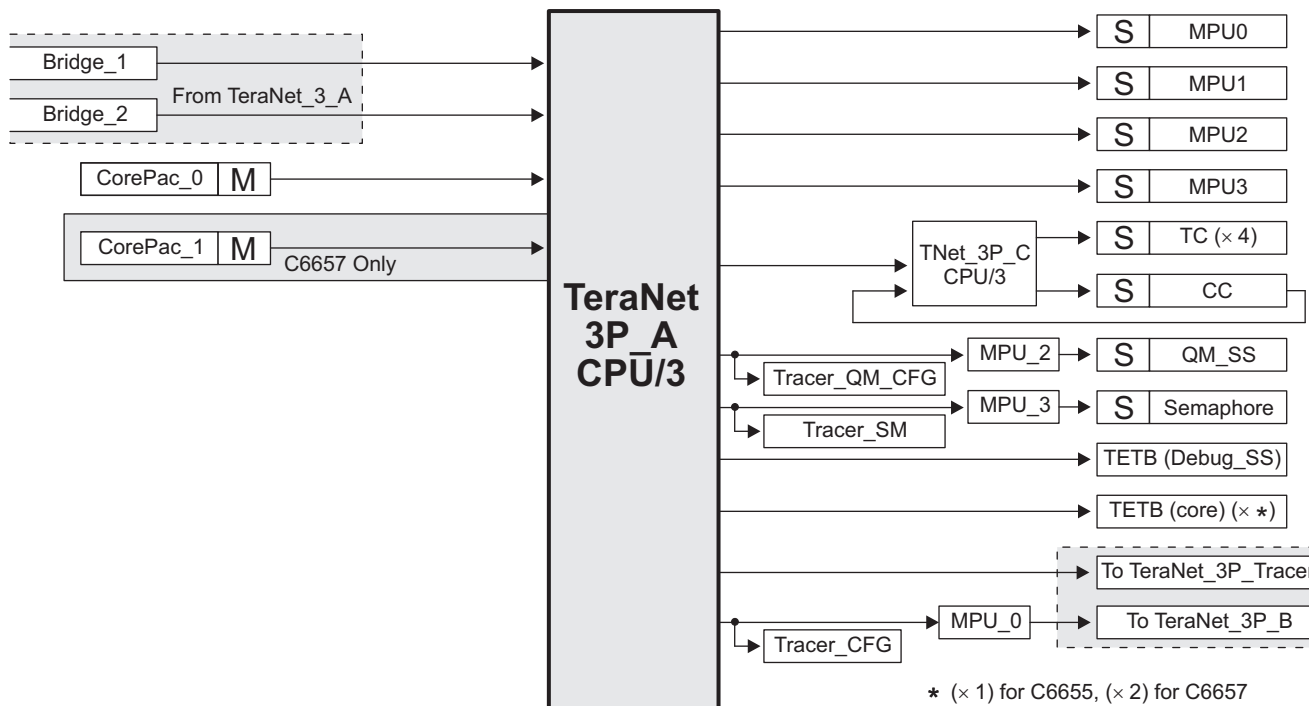
Figure 9-2. TeraNet 3P_A
