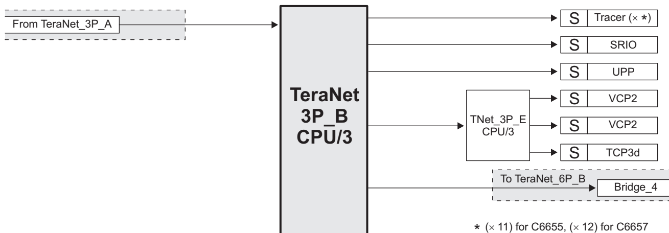
Figure 9-3. TeraNet 3P_B
