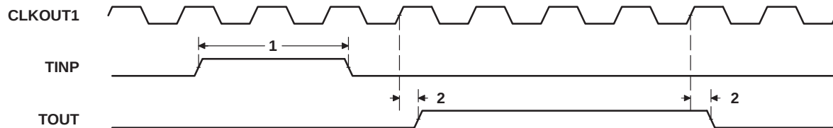
Figure 40. Timer Timing
