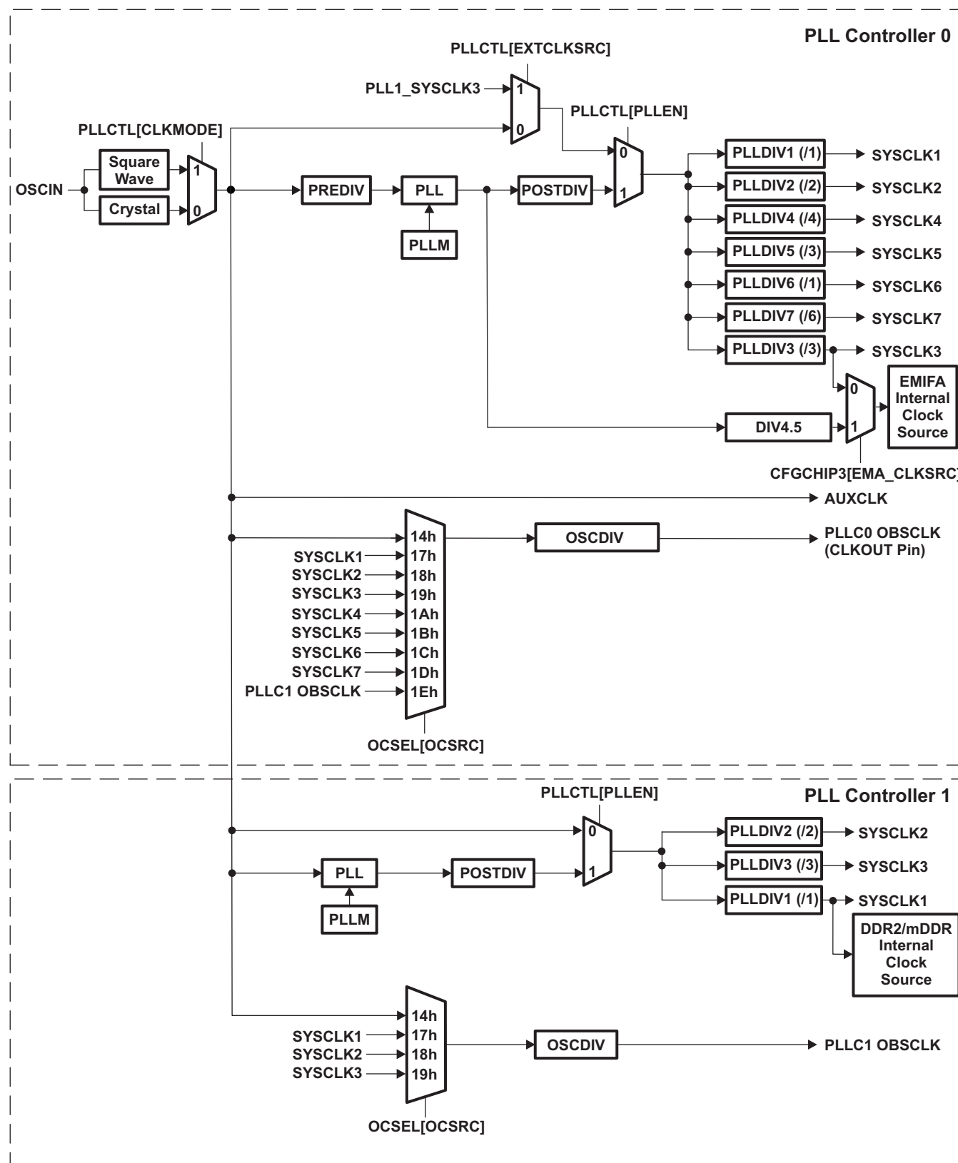
Figure 6-9. PLL Topology
