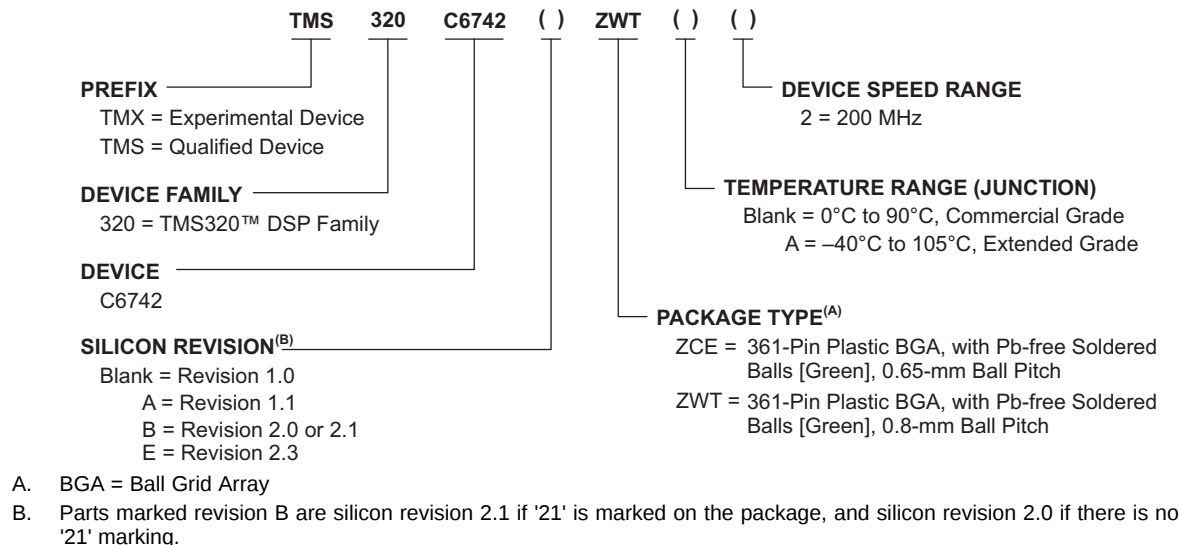
Figure 7-1. Device Nomenclature
