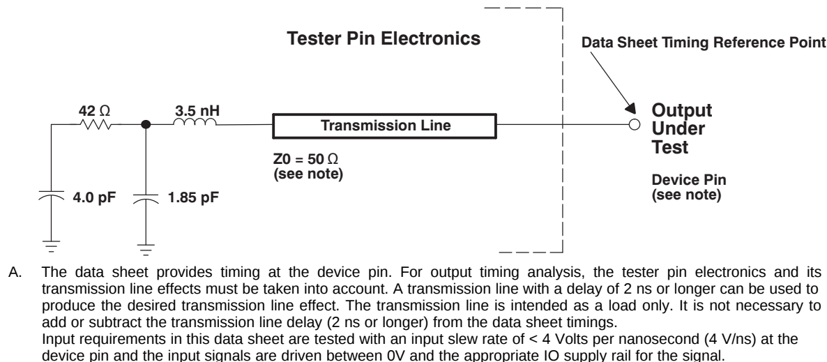
Figure 6-1. Test Load Circuit for AC Timing Measurements
