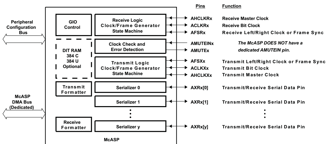
Figure 6-26. McASP Block Diagram
