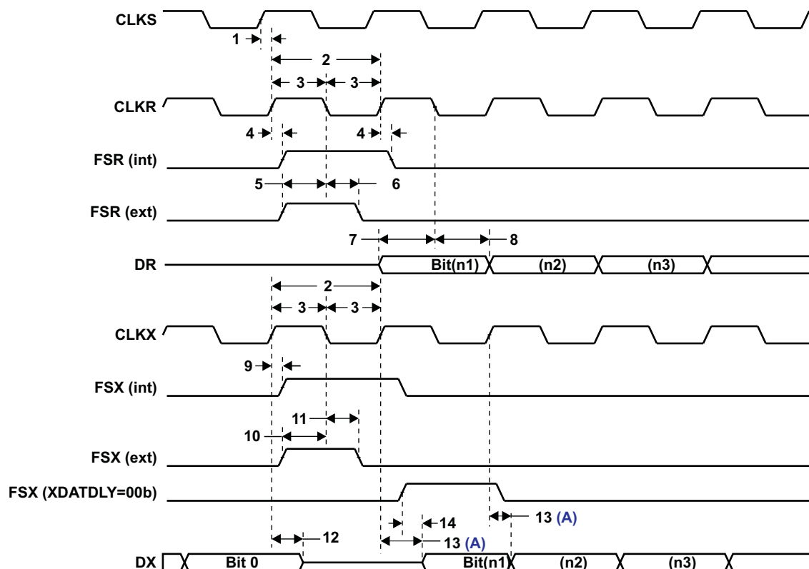
Figure 6-29. McBSP Timing
