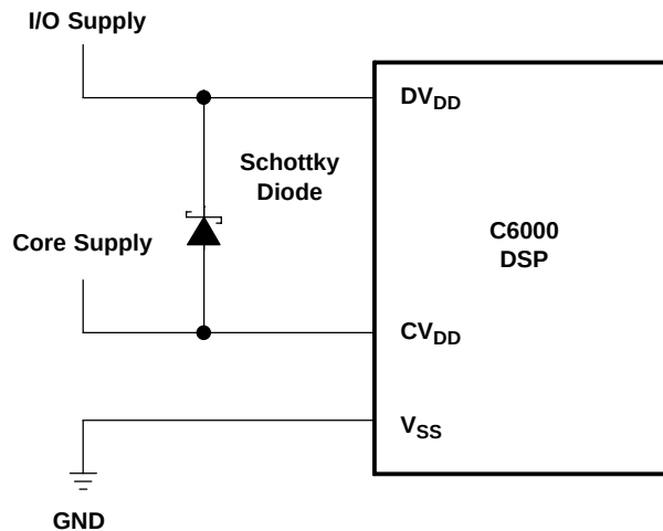
Figure 4–7. Schottky Diode Diagram
