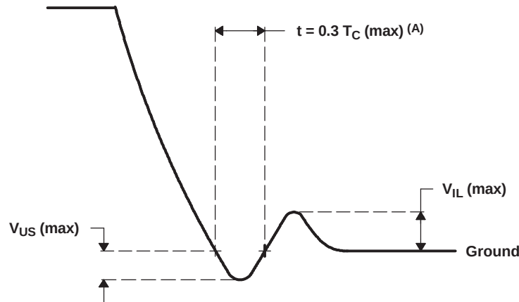
Figure 5-5. AC Transient Specification Fall Time
