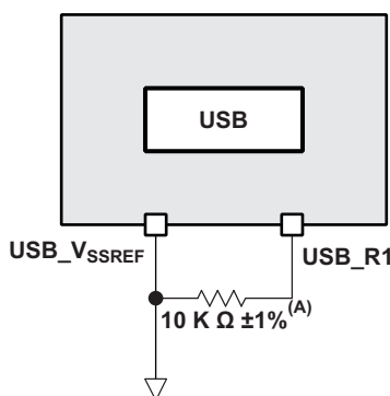
Figure 6-57. USB Reference Resistor Routing
