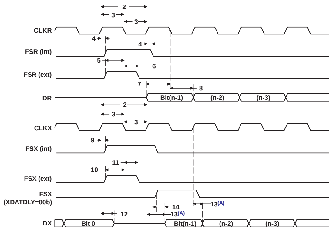
Figure 6-63. ASP Timing
