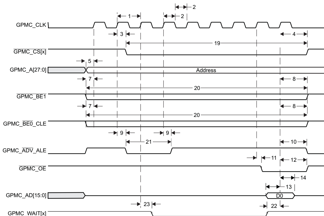
Figure 9-21. GPMC Non-Multiplexed NOR Flash - Synchronous Single Read (GPMCCLKDIVIDER = 0)
