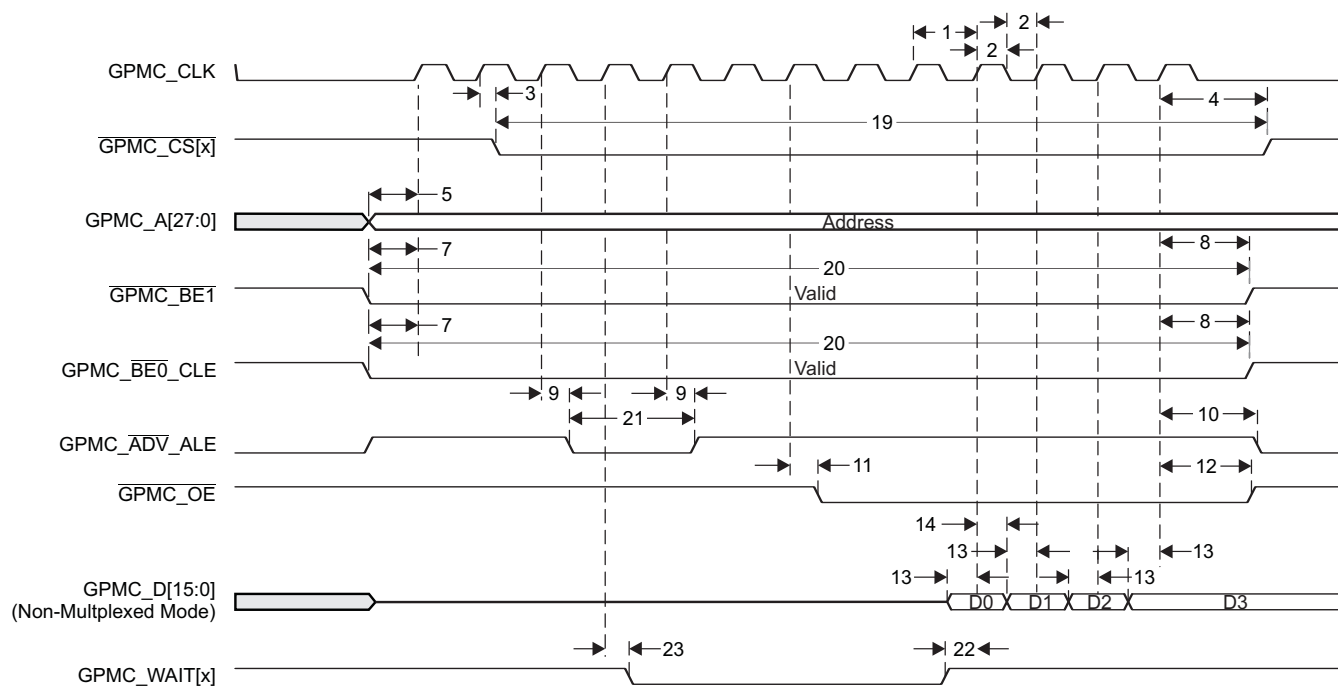
Figure 9-22. GPMC Non-Multiplexed NOR Flash - 14x16-bit Synchronous Burst Read (GPMCCLKDIVIDER = 0)
