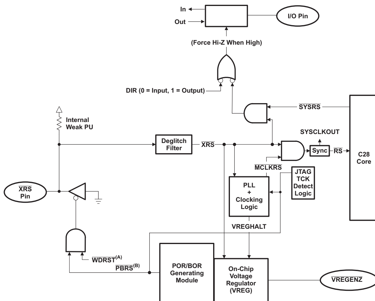
Figure 2-3. VREG + POR + BOR + Reset Signal Connectivity
