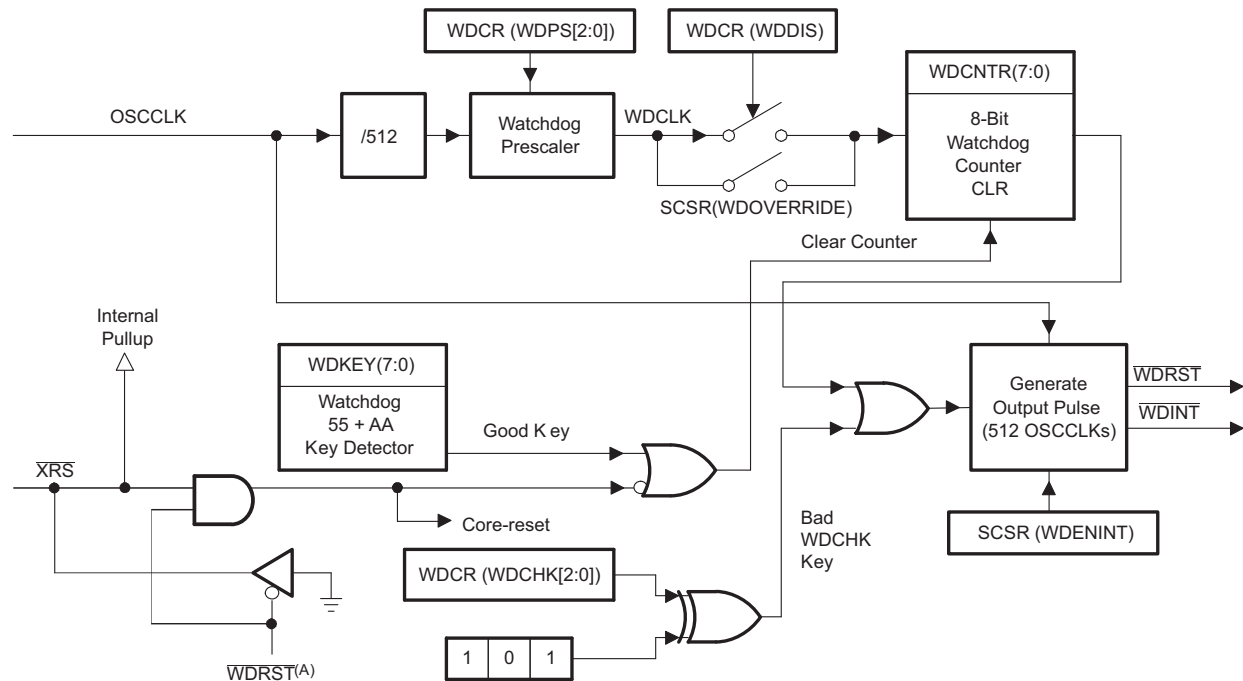
Figure 6-21. Watchdog Module
