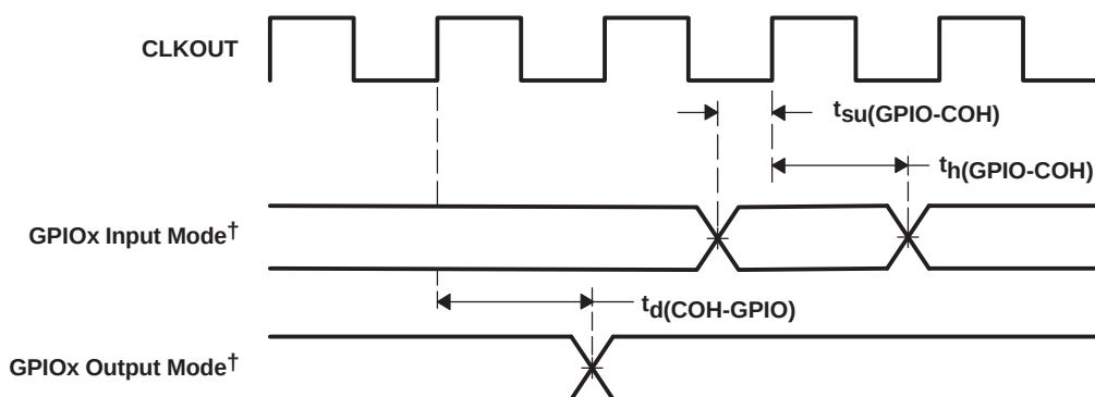
Figure 5-31. \text{GPIOx}^\dagger Timings
