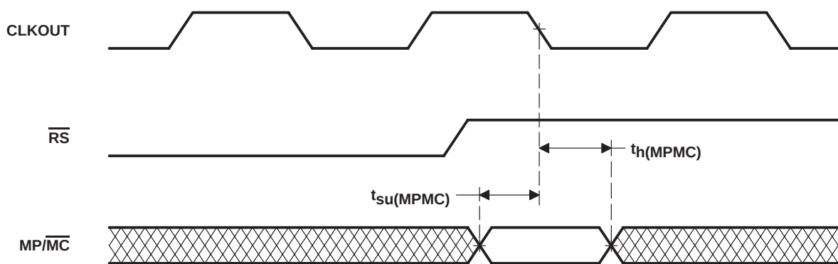
Figure 5-17. \overline{\text{MP/MC}} Timing
