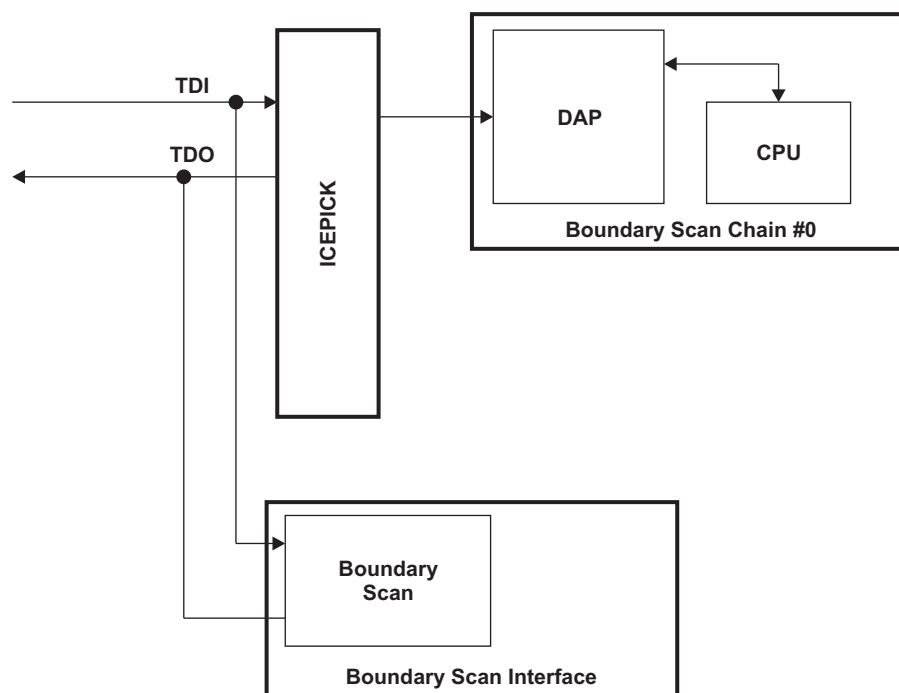
Figure 3-1. Debug Scan Chains
