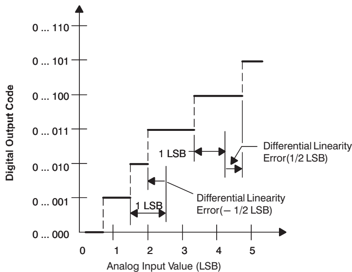
Figure 23. Differential Nonlinearity (DNL)
