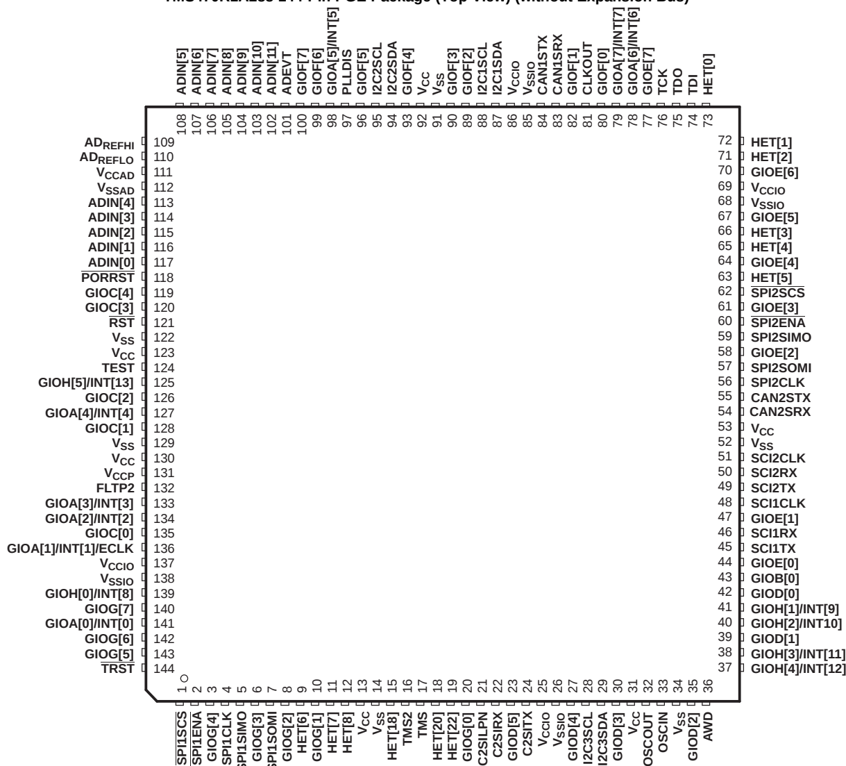
TMS470R1A288 144-Pin PGE Package (Top View) (without Expansion Bus)
