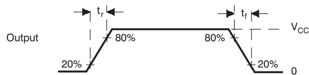
Figure 10. CMOS-Level Outputs
