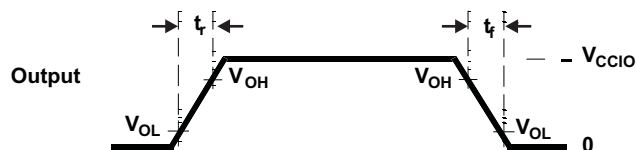
Figure 4-5. CMOS-Level Outputs
