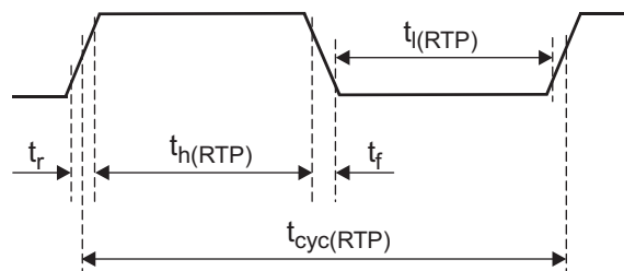
Figure 5-32. RTPCLK Timing
