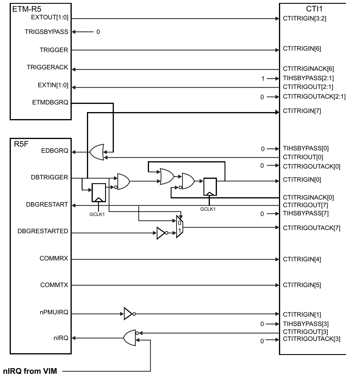
Figure 5-25. CTI1 Mapping
