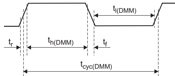
Figure 5-35. DMMCLK Timing
