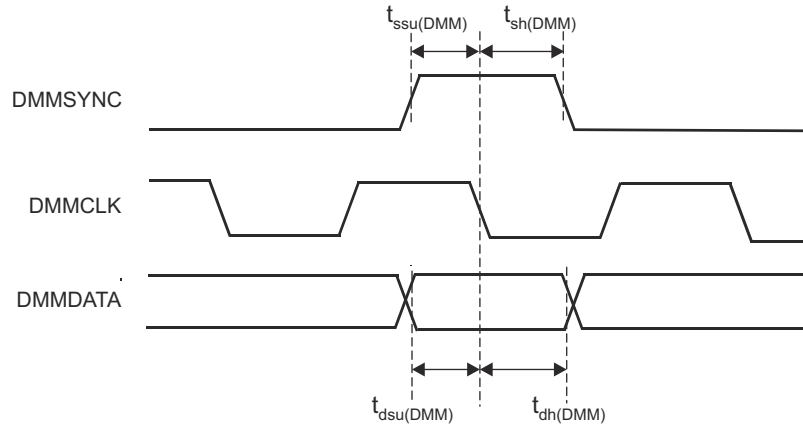
Figure 7-36. DMMDATA Timing
