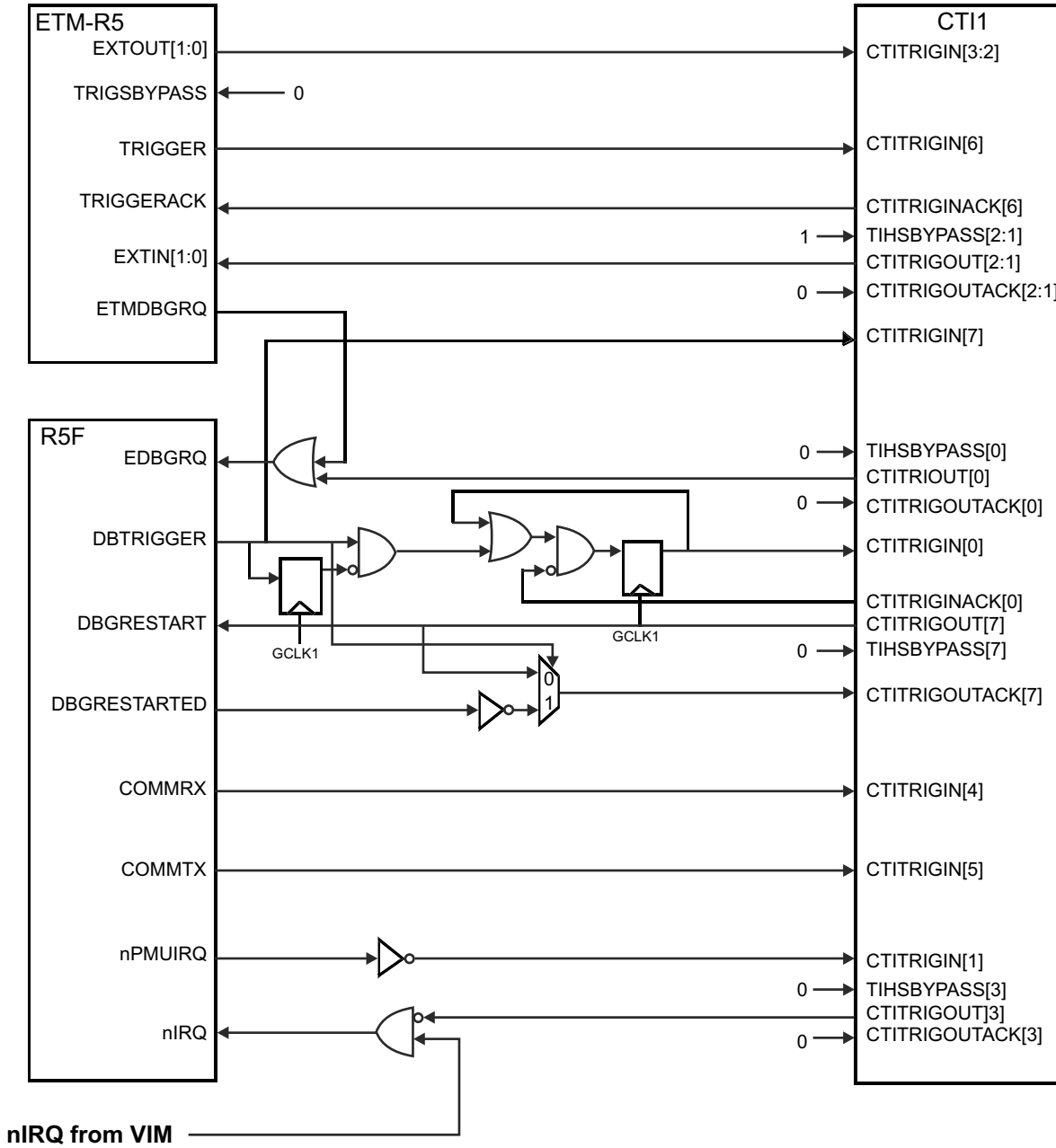
Figure 7-25. CTI1 Mapping
