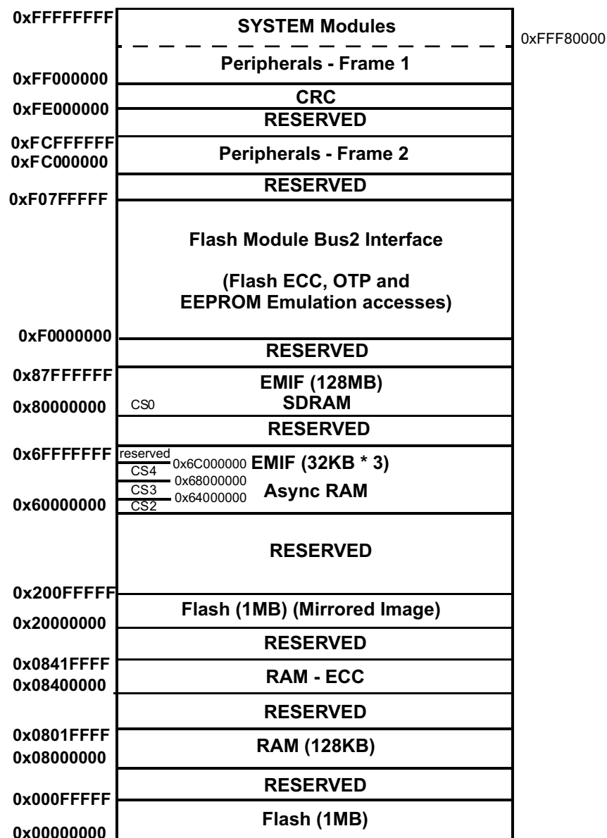
Figure 6-10. Memory Map
