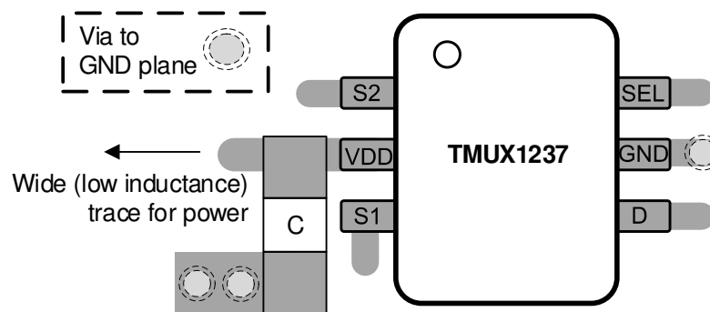
Figure 22. TMUX1237 Layout Example
