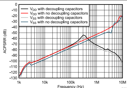
Figure 6-26. ACPSR vs Frequency
