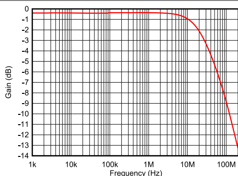
Figure 6-25. On Response vs Frequency
