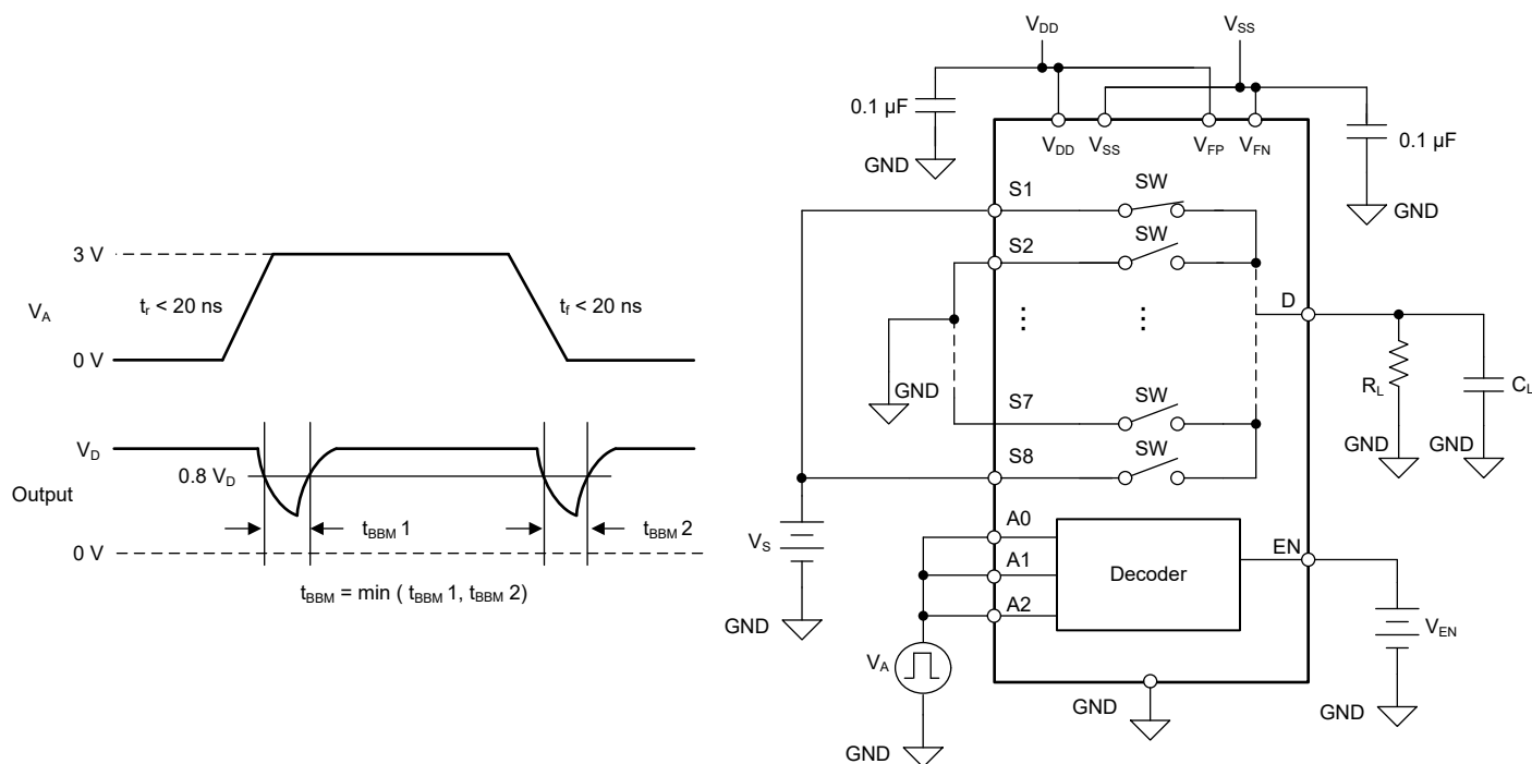
Figure 8-6. Break-Before-Make Delay Measurement Setup
