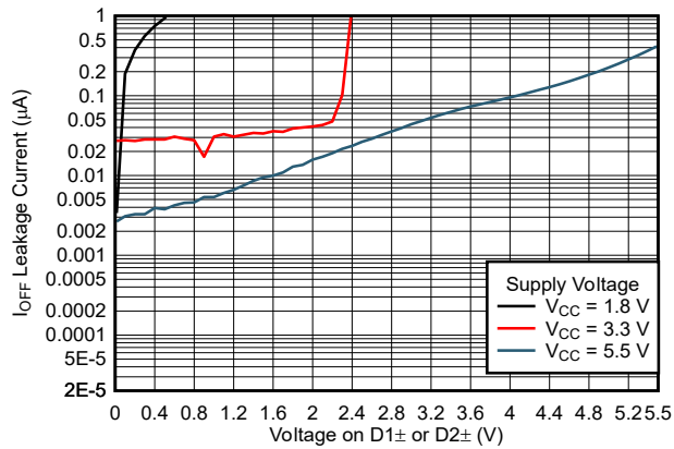
Figure 6-13. I OFF Leakage Current vs Voltage on D1± or D2±
