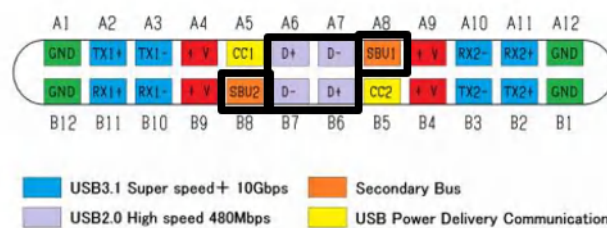
Figure 7-1. USB Type-C Connector Pinout
