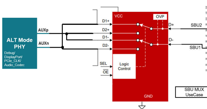
SBU Pins Application Use Case
