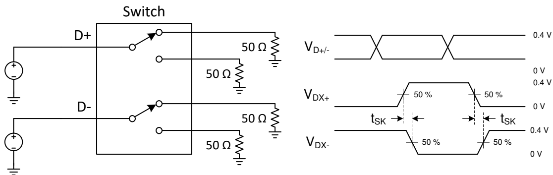
Figure 6-9. t_{PD}
