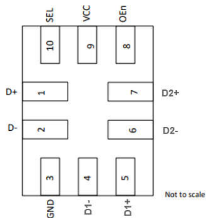
Figure 4-1. RSW Package 10-Pin UQFN (Top View)
