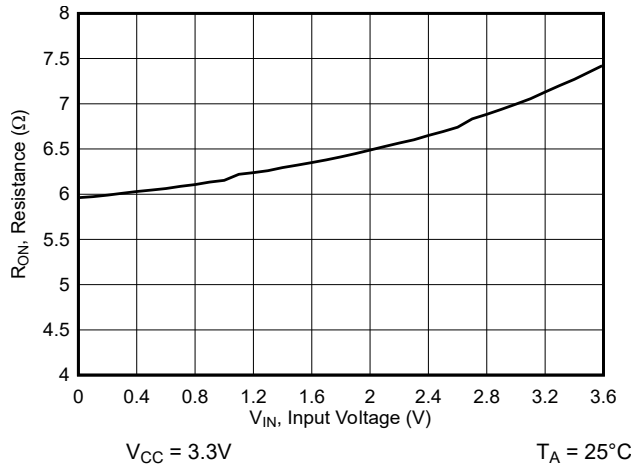
Figure 6-11. ON-Resistance vs Input Voltage
