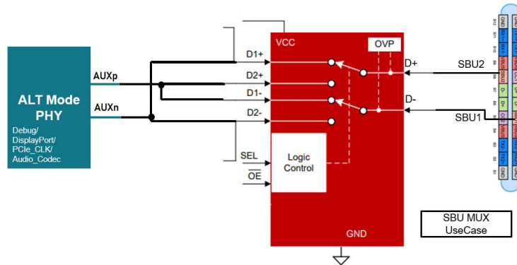
Figure 7-4. SBU Use Case
