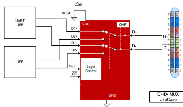
Figure 8-2. Typical TMUXHS221F Application - D+/D- Use case
