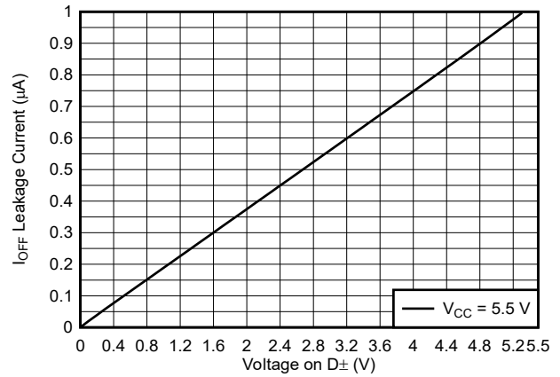
Figure 6-12. I OFF Leakage Current vs Voltage on D±
