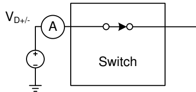
Figure 6-3. On Leakage
