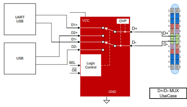
D+/D- Pins Application Use Case
