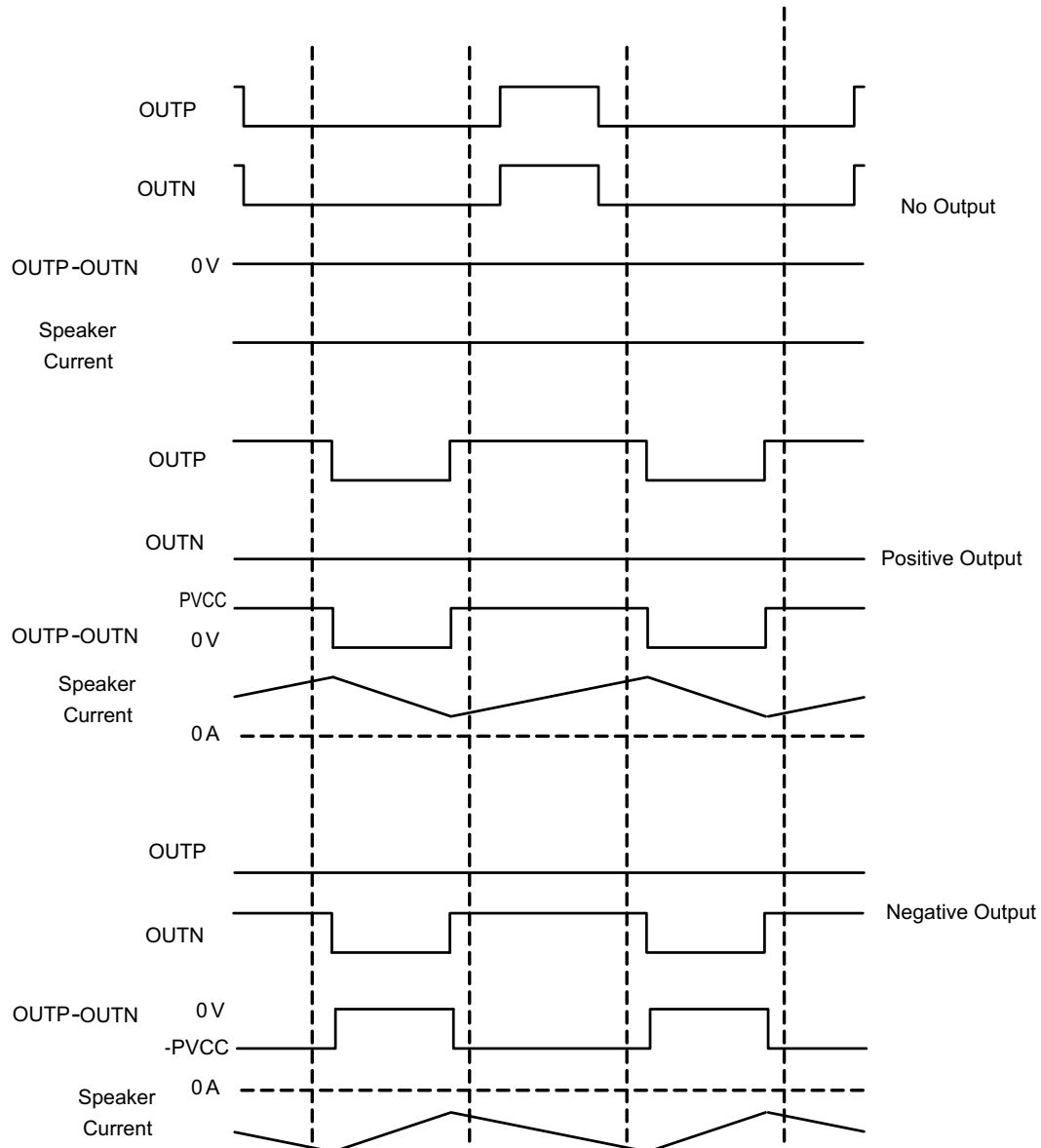
Figure 7-3. Low-Idle-Current 1SPW Modulation
