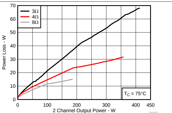
Figure 7. System Power Loss vs Output Power
