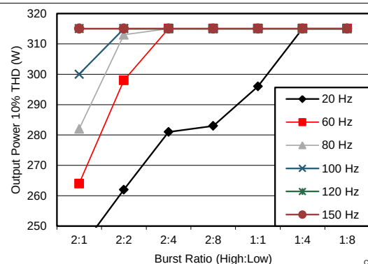
Figure 37. Maximum Burst Output Power vs Frequency, BTL, 4Ω Load, Each Channel, T_C = 75^\circ\text{C} , Power Ratio 1:8
